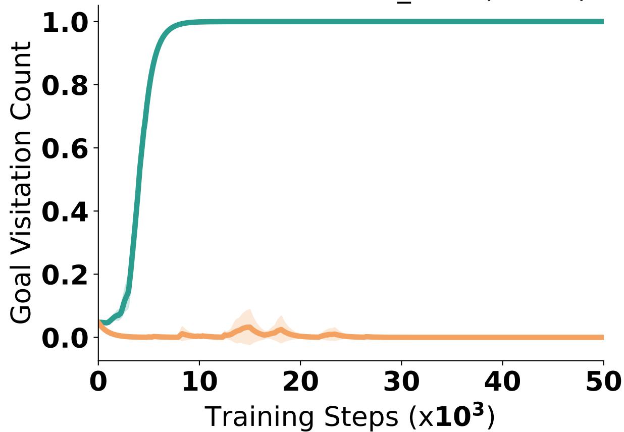
Gridworld-Bottleneck_Level(80.0%)
